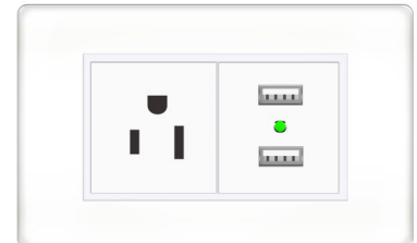
B-19 Contacto+ USB 6A/120-250v; 2.1A/5v DC
